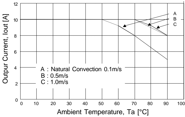
Derating ERS12-xxxx (SIL-11) at U_{in} = 3.3 \text{ Vdc} :
