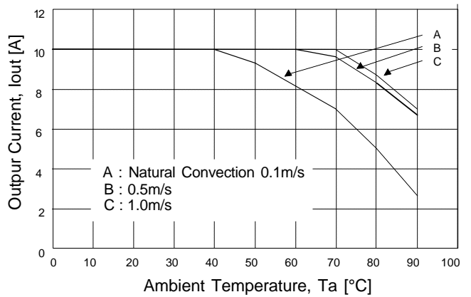
Derating ERS12-xxxx (SIL-11) at U_{in} = 5 \text{ Vdc} :
