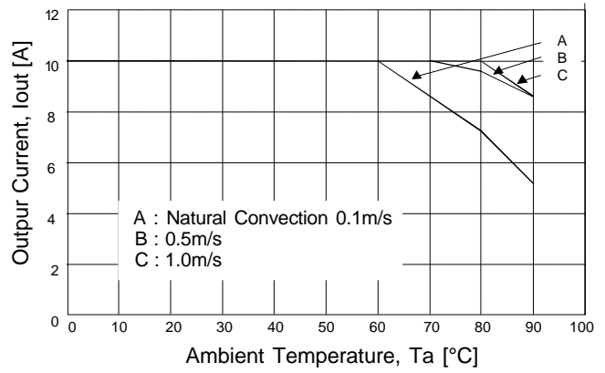
Derating ERS05-xxxx (SMD) at Uin =5 Vdc:
