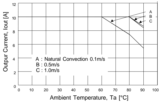
Derating ERS12-xxxx (SIL-11) at U_{in} = 5 \text{ Vdc} :
