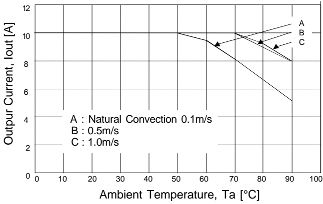
Derating ERS05-xxxx-S (SMD) at Uin =3.3 Vdc:
