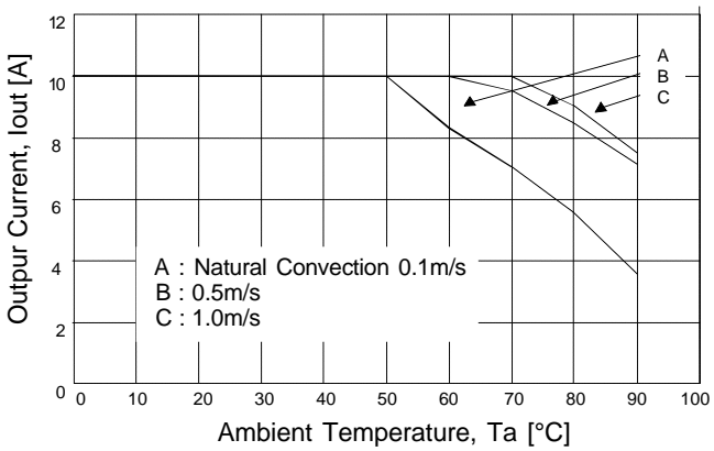
Derating ERS12-xxxx-S (SMD) at Uin =3.3 Vdc:
