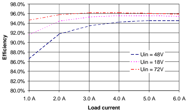
Efficiency U_{out} = 3.3V (typical)
