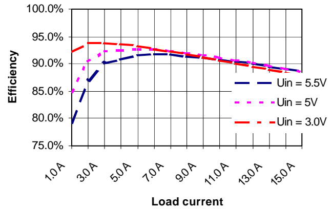
Efficiency U_{out} = 1.8V (typical)
