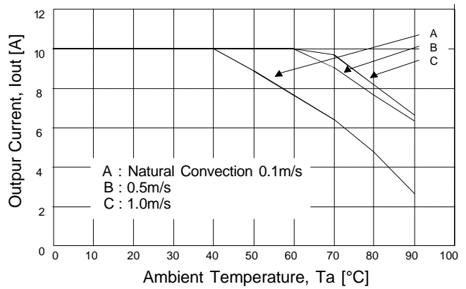
Derating ERS12-xxxx (SMD) at Uin =5 Vdc:
